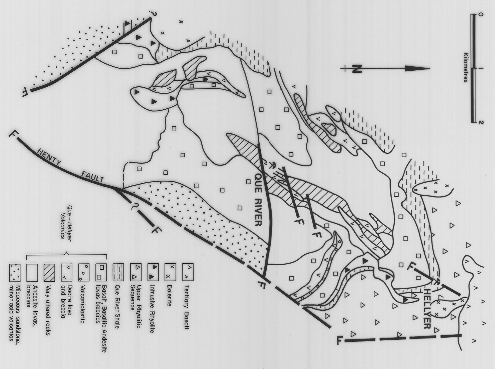
FIG. 1 QUE - HELLYER VOLCANICS REGIONAL GEOLOGY
