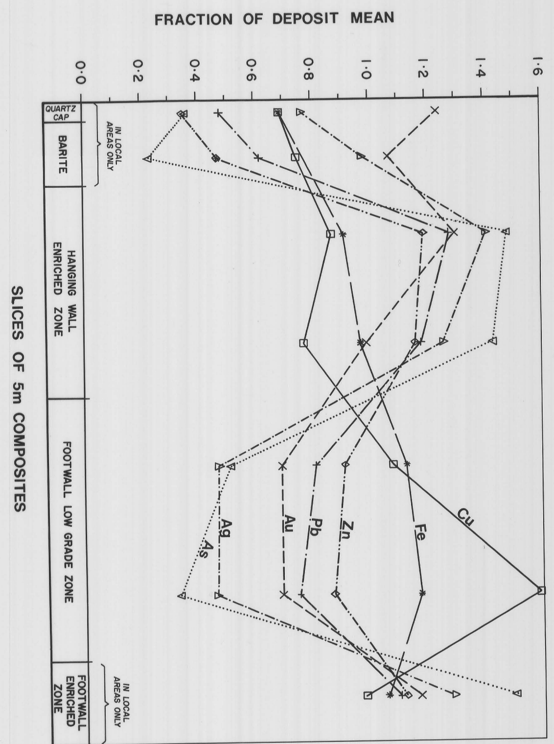
FIG. 3 HELLYER - STRATIGRAPHIC METAL ZONING
