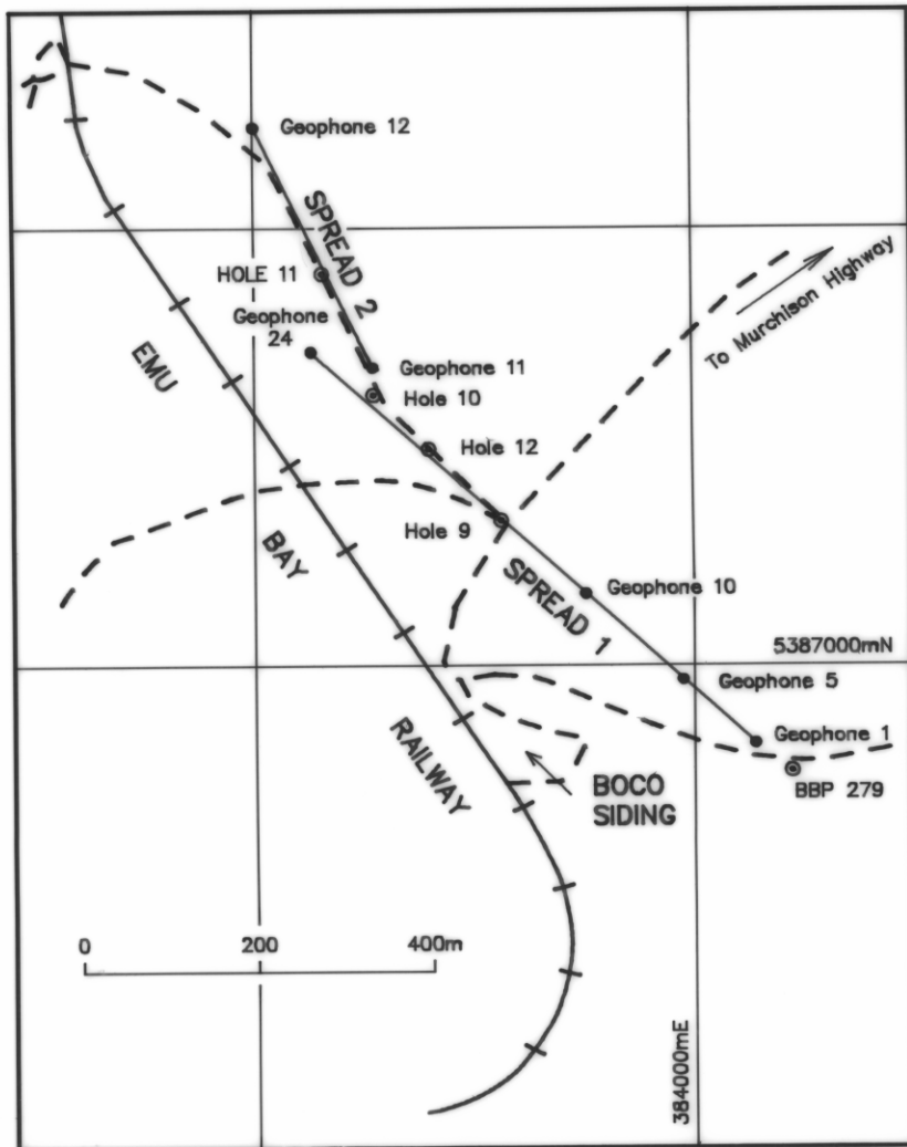
BOCO SIDING LOCALITY PLAN
