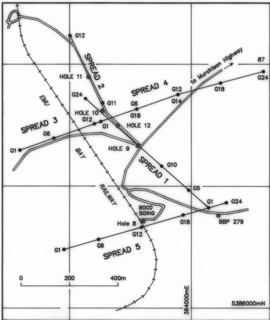
BOCO SIDING - LOCALITY PLAN OF SEISMIC SPREADS FIGURE No. U/R 1989/05 AUTHOR: R.G. RICHARDSON TASMANIA DEPARTMENT OF MINES, DRAFTSPERSON: J. LADANIWSKYJ 5192 C
