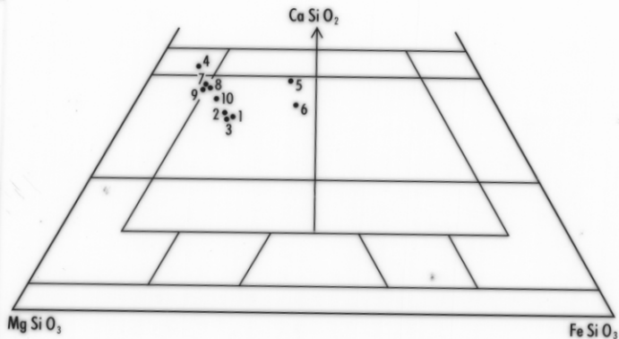
Fig. 22 : Pyroxene quadrilateral showing the composition of clinopyroxene from tholeiitic basalt within the Crimson Creek Formation. Plot numbers refer to analyses (table 6)
