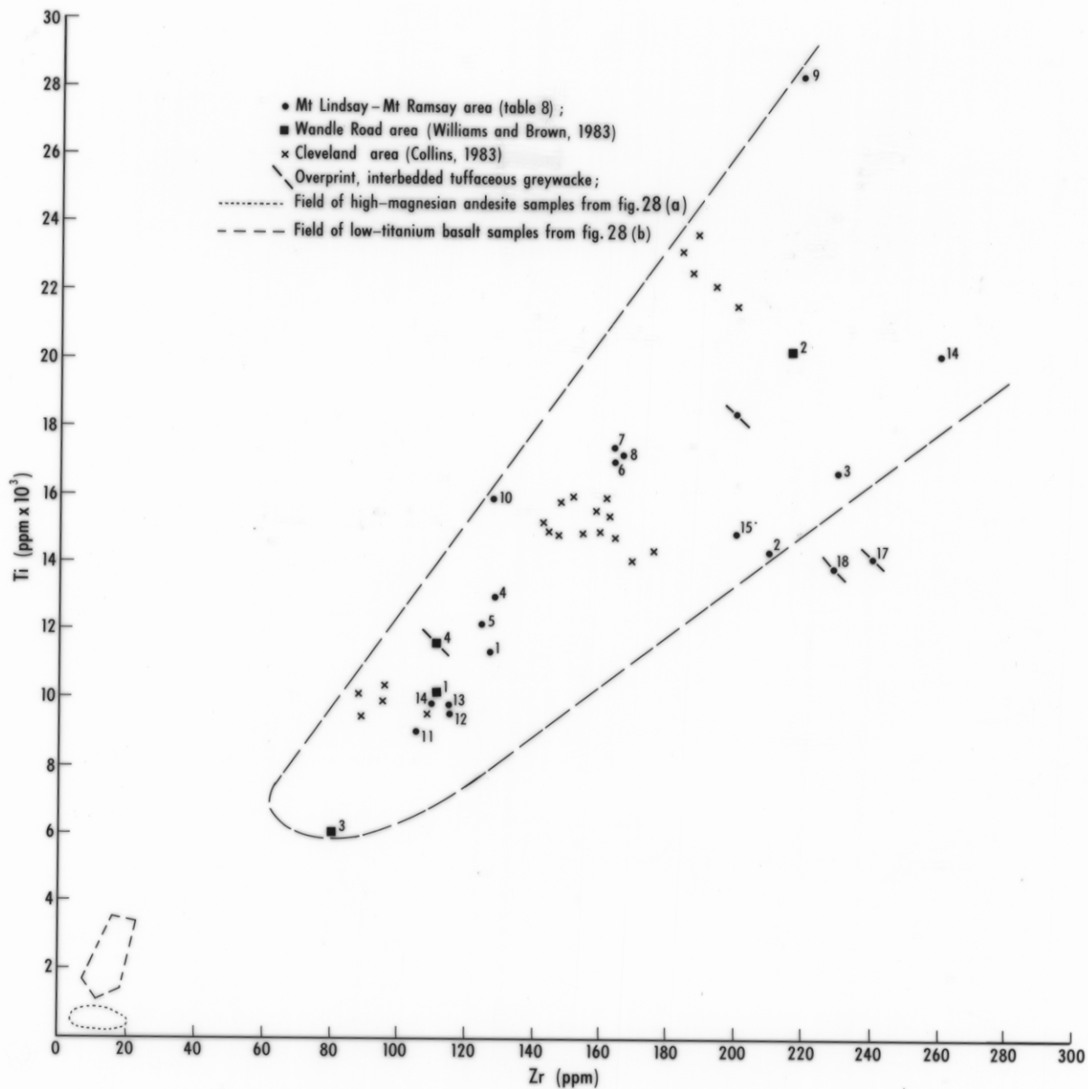
Fig. 28 (c): Ti-Zr discriminant diagram for basalt samples from the Crimson Creek Formation and correlates in the Dundas-Waratah region.
