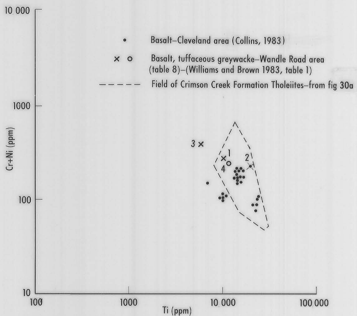
Fig 30b: (Cr+Ni) ~ Ti diagrams for samples from Crimson Creek Formation correlates in the Cleveland-Arthur River area
