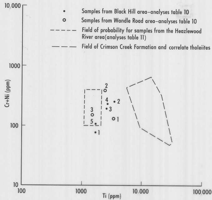
Fig 30c: (Cr+Ni) ~ Ti discriminant diagram for low-titanium basalt samples
