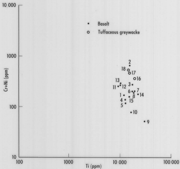
Fig 30a: (Cr+Ni) ~ Ti discriminant diagram of Crimson Creek Formation tholeiite samples from the extended type area, analyses table 8
