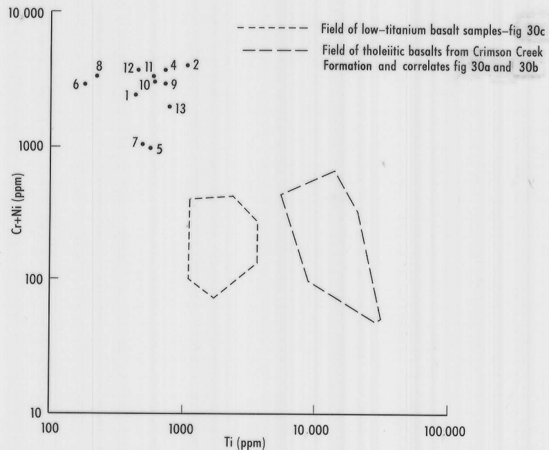
Fig 30d: (Cr+Ni) ~ Ti discriminant diagram for high magnesium andesite samples-analyses table 9
