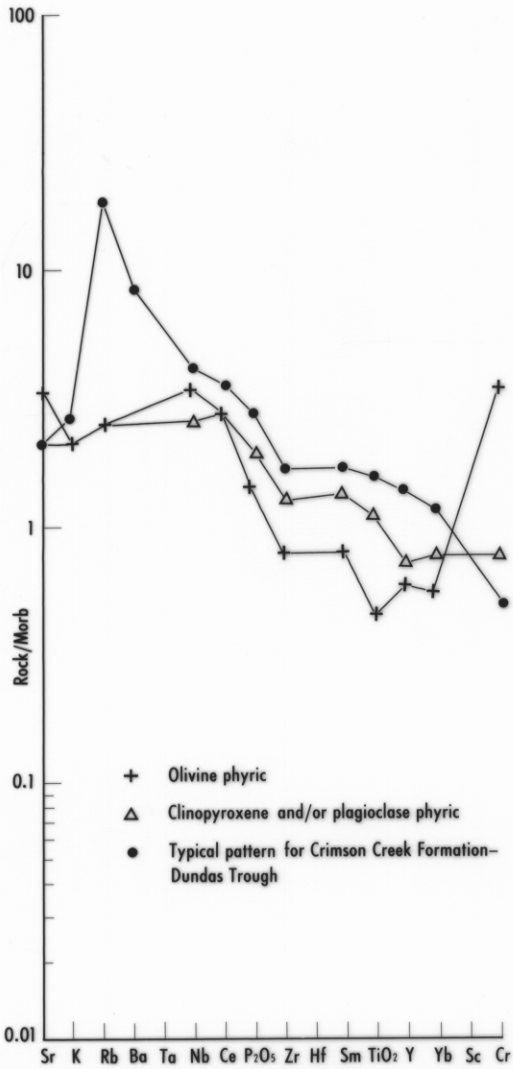
Fig 35: Geochemical pattern of Crimson Creek Formation correlate basalt in the Smithton Basin
