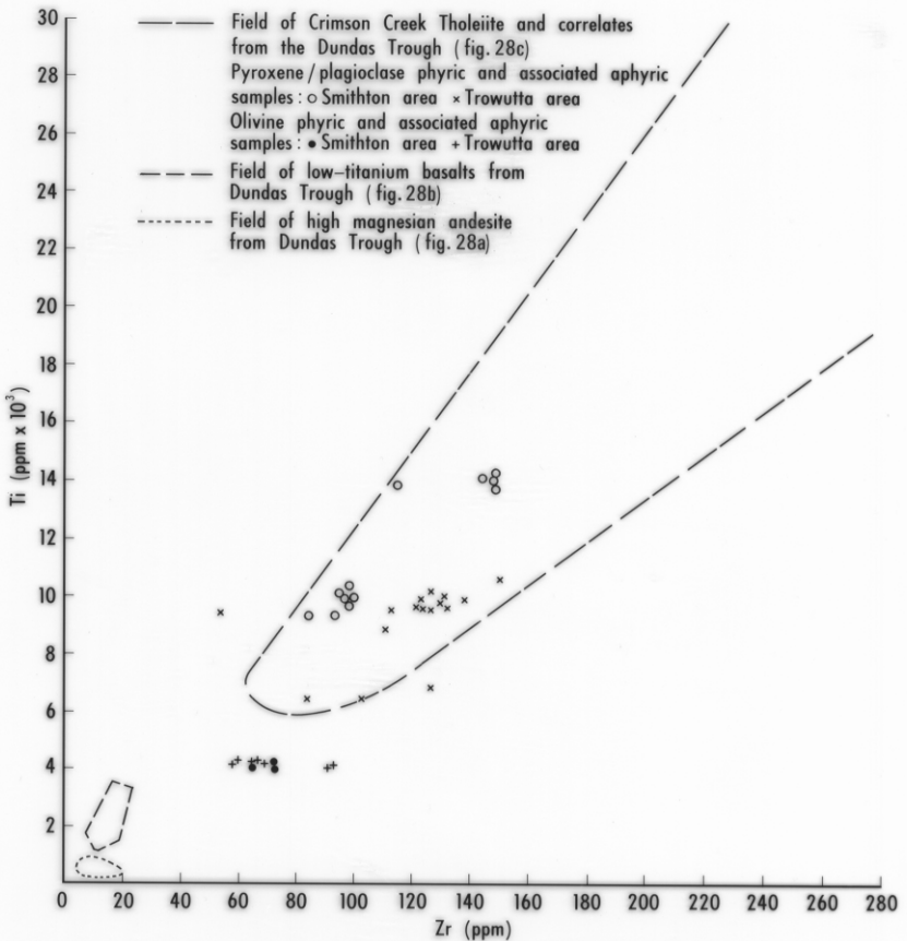
Fig. 36 : Ti Zr discriminant diagram for basaltic rocks from within Crimon Creek formation correlates in the Smithton Basin
