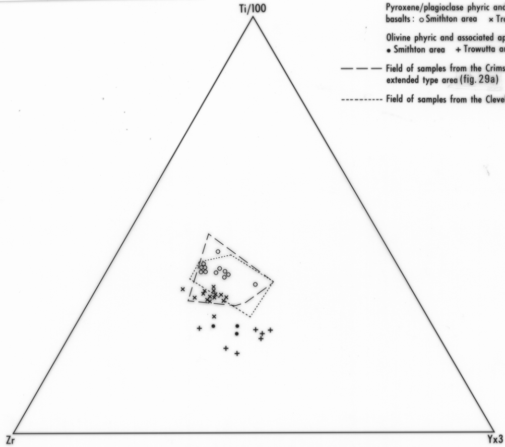
Fig. 37 : Ti~Y~Zr discriminant diagram for basaltic rocks from within the Crimson Creek Formation correlates in the Smithton Basin
