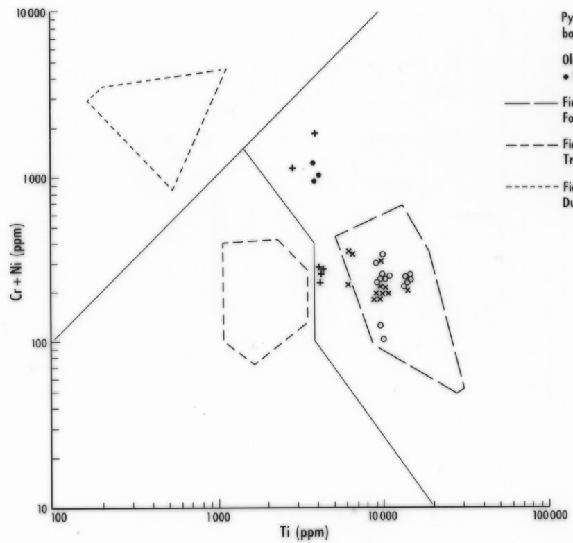
Fig. 38 : (Cr + Ni) ~ Ti discriminant diagram for basaltic rocks from within the Crimson Creek Formation correlates in the Smithton Basin
