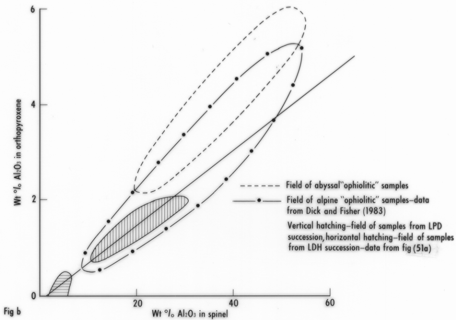
Fig 51a: Variation in Al_2O_3 in coexisting orthopyroxene and spinel
