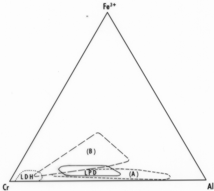
Fig. 53(b): Field of spinel compositions from the LDH and LPD successions compared with fields of spinel composition from a non Fe 3+ increasing body (A) (Josephine Peridotite, Dick 1977): and an Fe 3+ increasing body (B) (Marum Peridotite, Jaques 1981)
