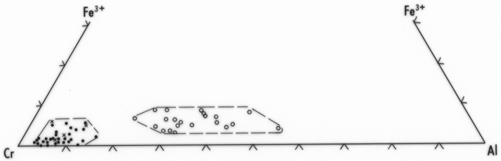
Fig. 53(a): Cr-Al-Fe 3+ plot of chrome spinel grains from the LDH succession: • dunite, pyroxene bearing dunite and harzburgite; × massive orthopyroxenite; ○ and LPD succession
