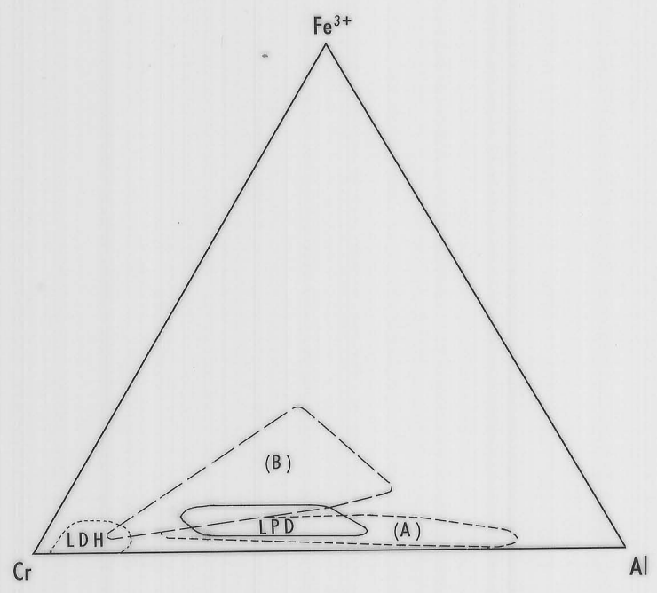
Fig. 53 (b): Field of spinel compositions from the LDH and LPD successions compared with fields of spinel composition from a non Fe 3+ increasing body (A) (Josephine Peridotite, Dick 1977): and an Fe 3+ increasing body (B) (Marum Peridotite, Jaques 1981)
