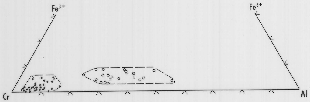
Fig. 53 (a): Cr-Al-Fe 3+ plot of chrome spinel grains from the LDH succession: • dunite, pyroxene bearing dunite and harzburgite; × massive orthopyroxenite; ○ and LPD succession
