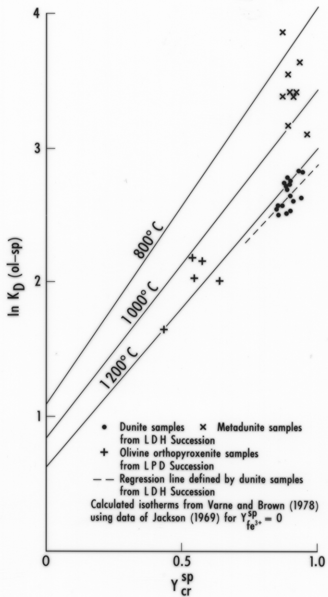
Fig.55 : \ln K_D(ol-sp) - Y_{cr}^{sp} for spinel samples from LDH and LPD Successions
