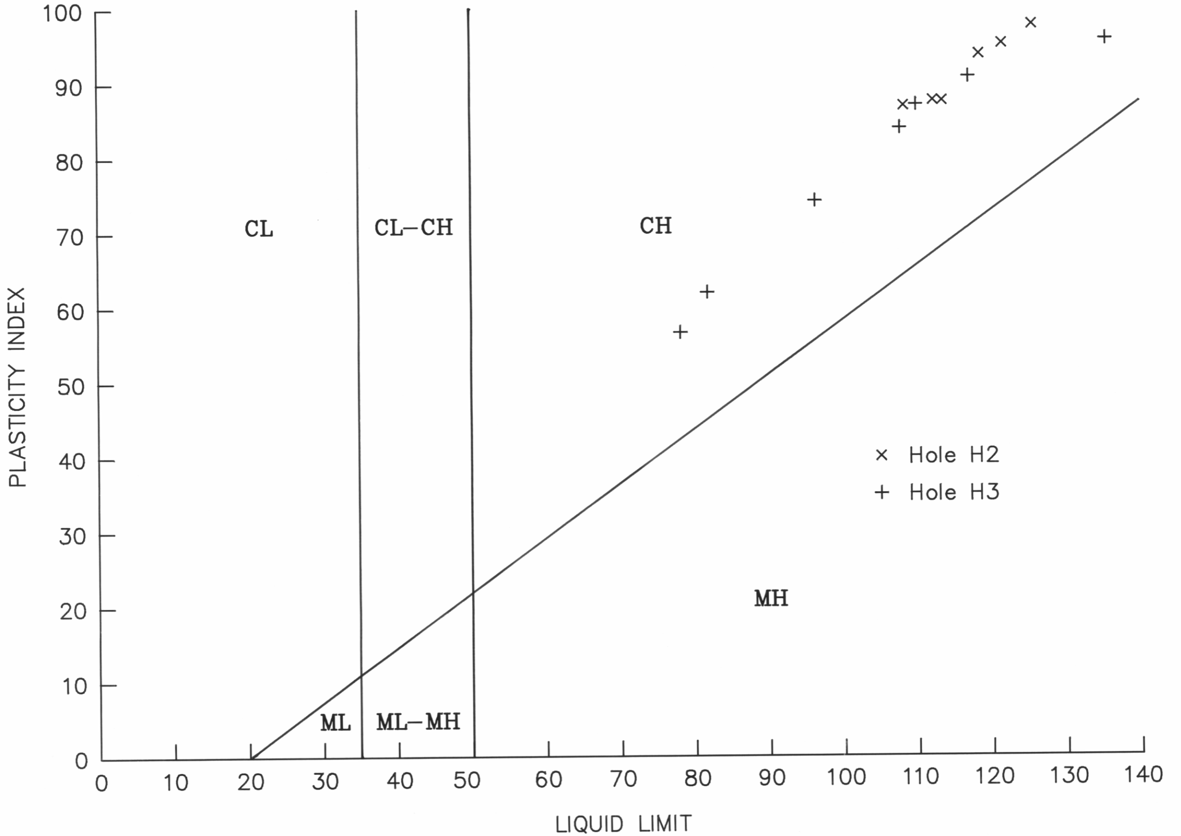
Figure. 2 Soil Laboratory Classification of the clays, Picketts house, Windermere W.R. Moore
