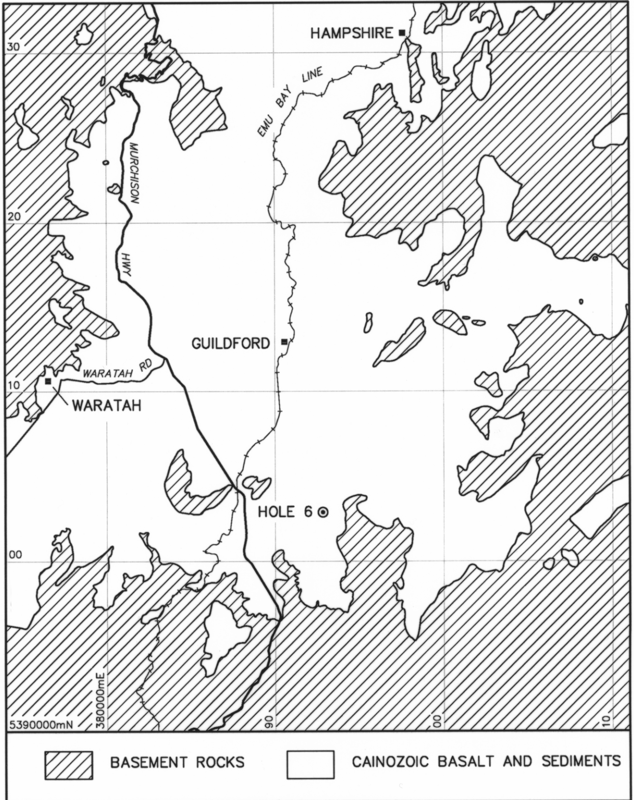
LOCATION MAP OF DRILL HOLES MT READ PROJECT - SUB-BASALT DRILLING PROJECT TASMANIA DEPARTMENT OF MINES U/R 1987/44 - P.W.BAILLIE, SEPT 1987 5234 E
