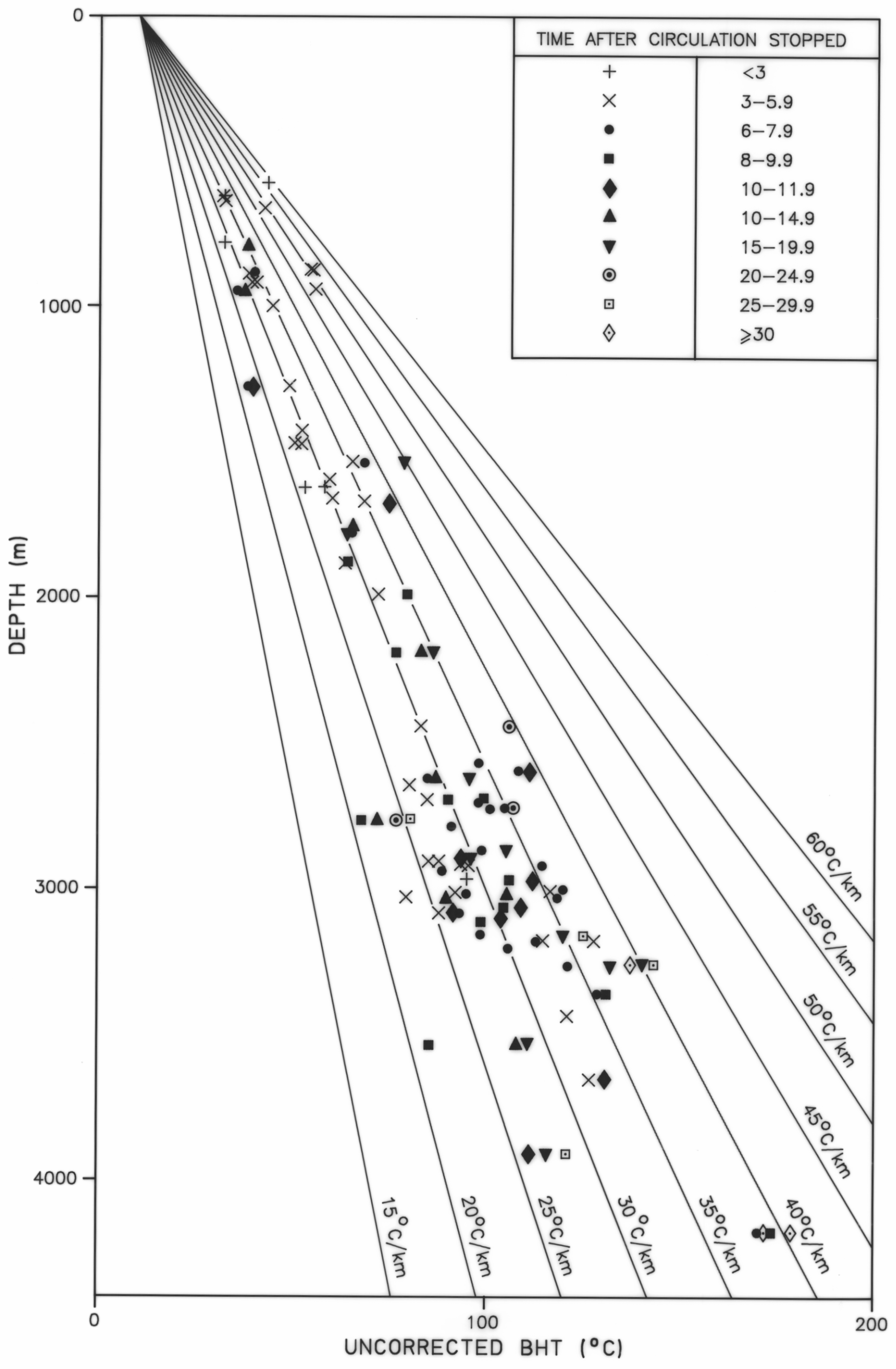
TASMANIAN EXPLORATION WELLS - DEPTH vs UNCORRECTED BHT (°C) TAS. DEPT. OF MINES PUBLISHED IN "APEA" Vol 29 1989, FIG. 2 AUTHOR: P.W. BAILLIE 5273 B
