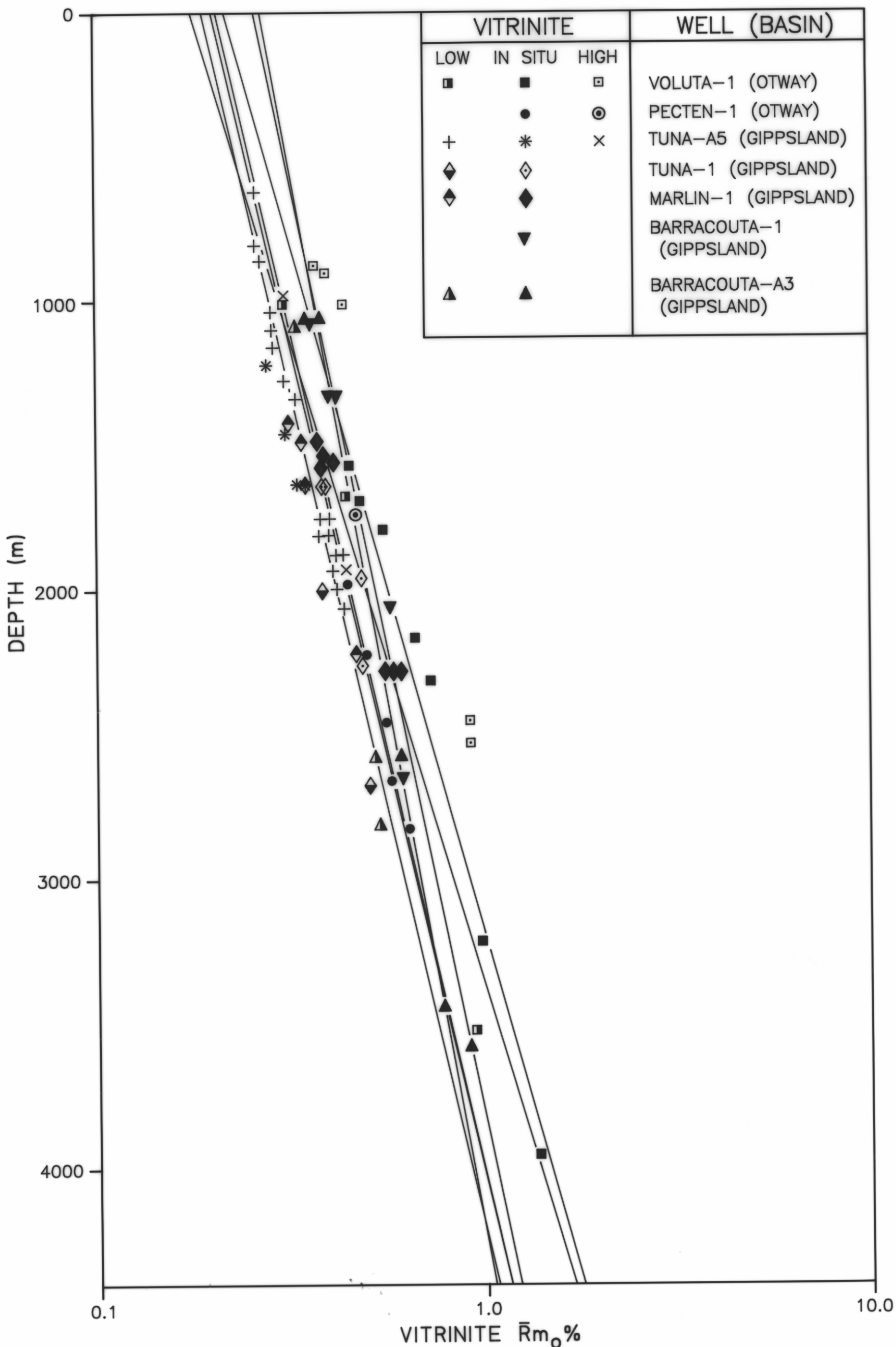
TASMANIAN OFFSHORE OIL WELLS - VITRINITE vs DEPTH/RM(0)% - NON TAS. PORTIONS OF GIPPSLAND & OTWAY BASINS TAS. DEPT. OF MINES PUBLISHED IN "APEA" Vol 29 1989, Fig. 8 AUTHOR: P.W. BAILLIE 5273 K
