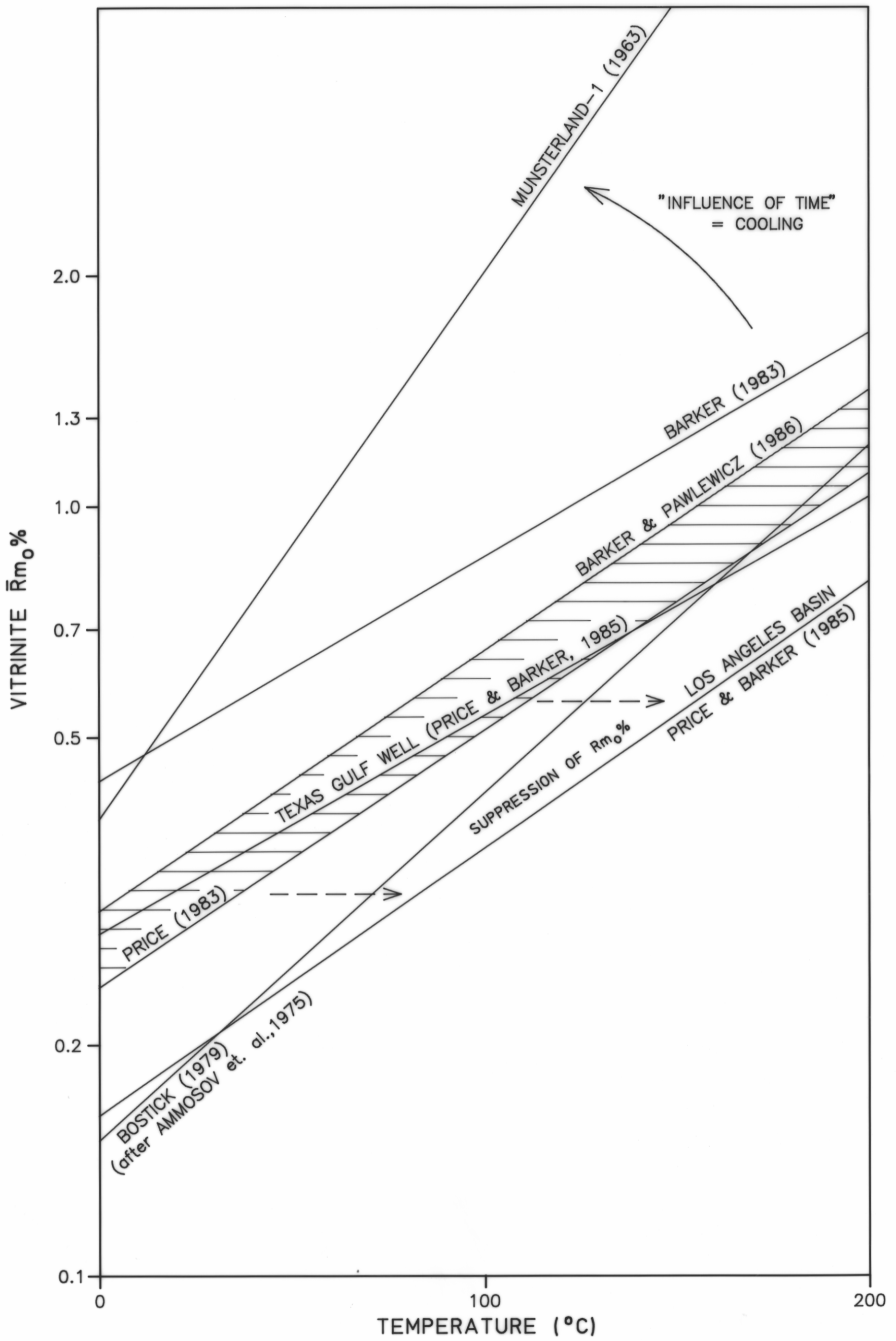
TASMANIAN OFFSHORE OIL WELLS - EXAMPLES OF VITRINITE vs TEMP. IN OTHER LITERATURE TAS. DEPT. OF MINES PUBLISHED IN "APEA" Vol 29 1989, Fig.B1 AUTHOR: P.W. BAILLIE 5273 L
