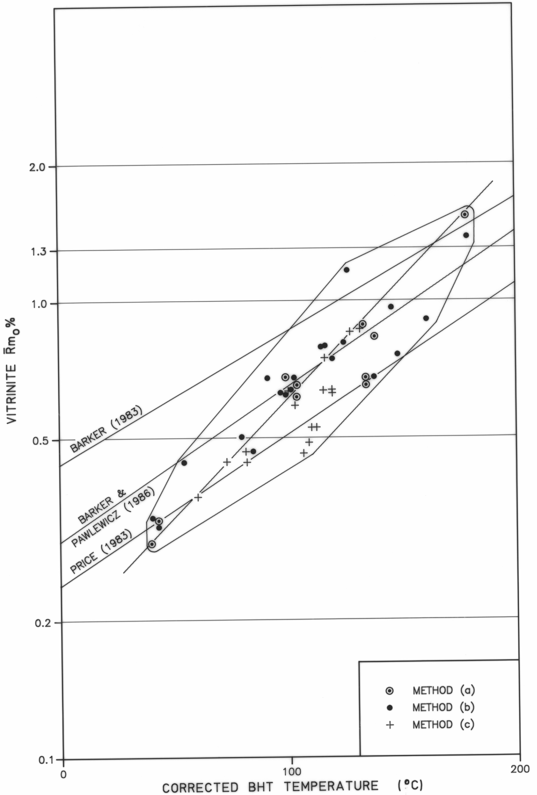
TASMANIAN EXPLORATION WELLS - VITRINITE vs TEMPERATURE / RM(0)% TRENDS TAS. DEPT. OF MINES PUBLISHED IN "APEA" Vol 29 1989, Fig.9 AUTHOR: P.W. BAILLIE 5273 M
