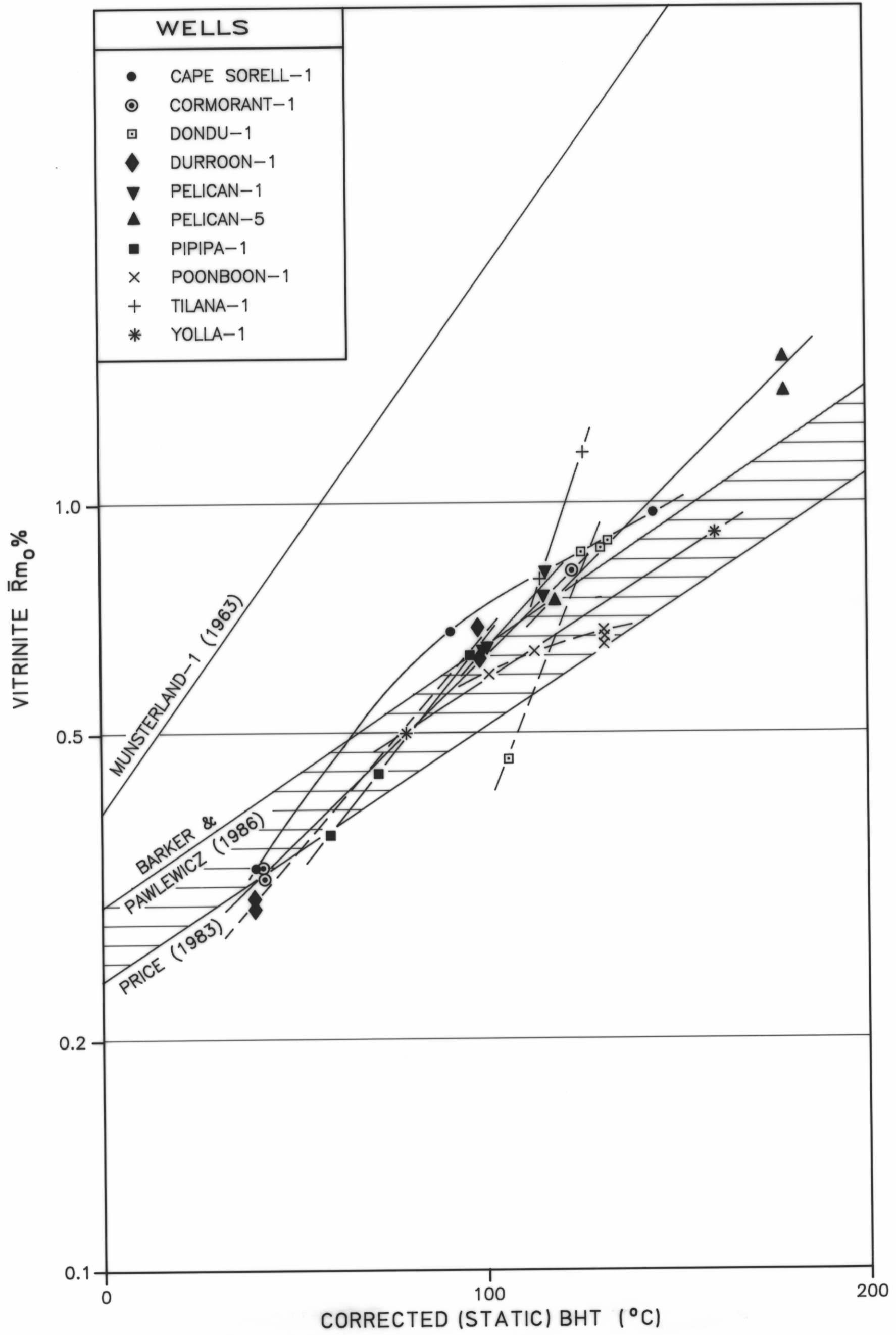
TASMANIAN OFFSHORE OIL WELLS - VITRINITE vs TEMPERATURE / REFLECTANCE TRENDS TAS. DEPT. OF MINES PUBLISHED IN "APEA" Vol 29 1989, Fig. 10 AUTHOR: P.W. BAILLIE 5273 N
