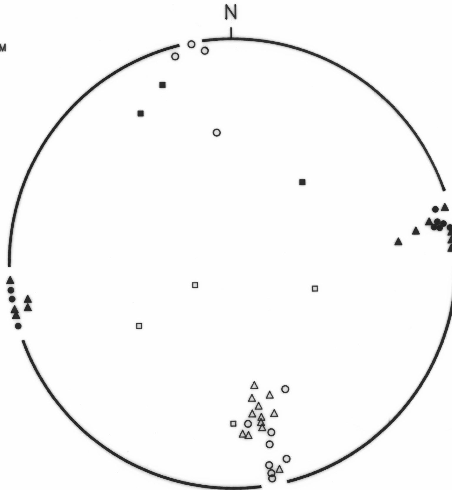
FIG. 1 Minor folds in the Twelvetrees Quartzite
