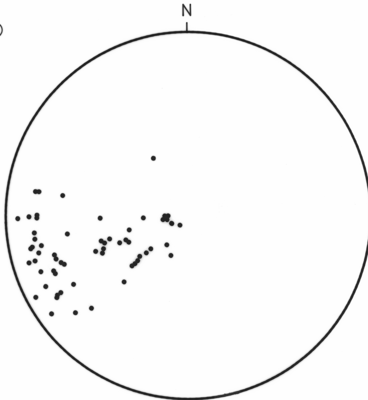
PWB 2 Poles to bedding - Parmeener Supergroup - Misery Range area
