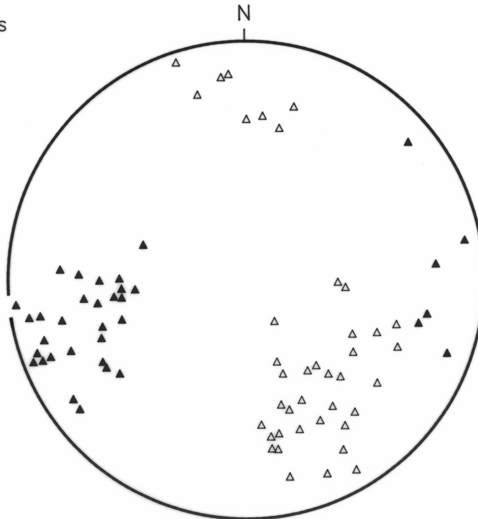
FIG. 2(a) Minor folds in the mixed-grey mica-quartz & quartz-mica phyllite east of the Twelvvetrees Range
