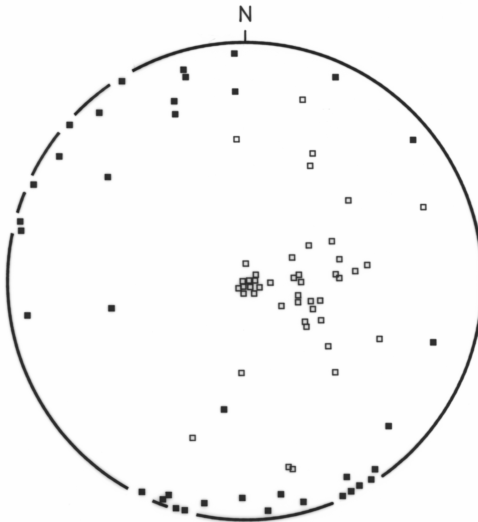
FIG. 2(b) Minor folds in the mixed grey mica-quartz & quartz-mica phyllite east of the Twelvvetrees Range
