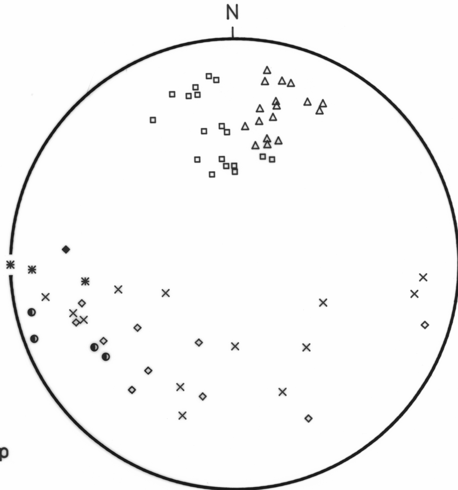
FIG. 5 Stereoplot of structural elements from domain 2
