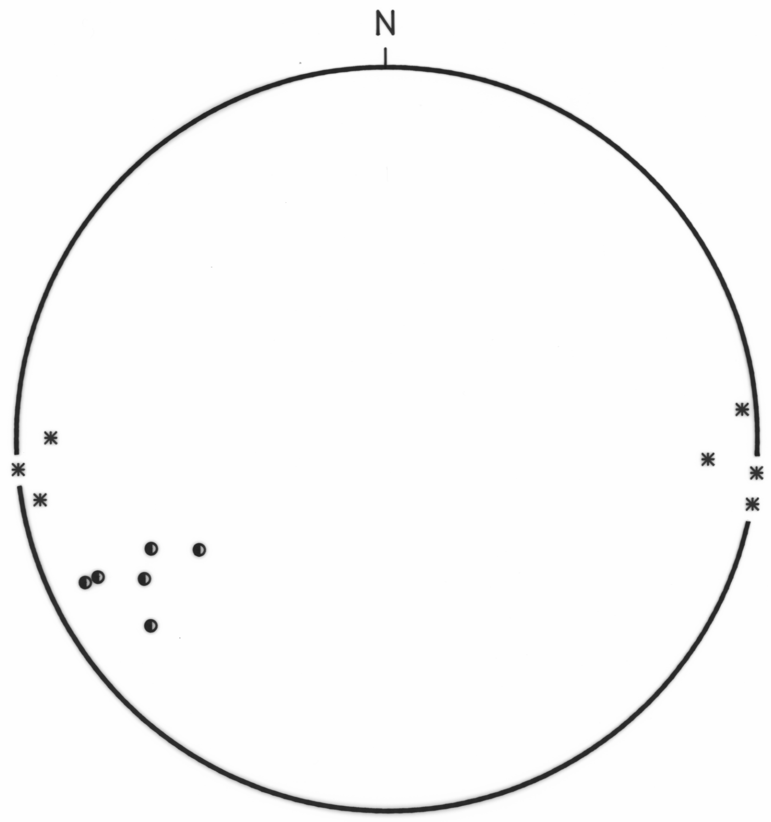
FIG. 6 Stereoplot of structural elements from domain 3
