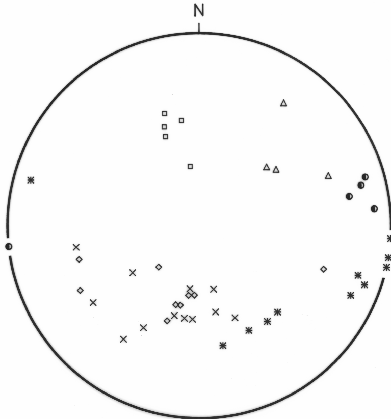
FIG. 8 Stereoplot of structural elements from domain 5
