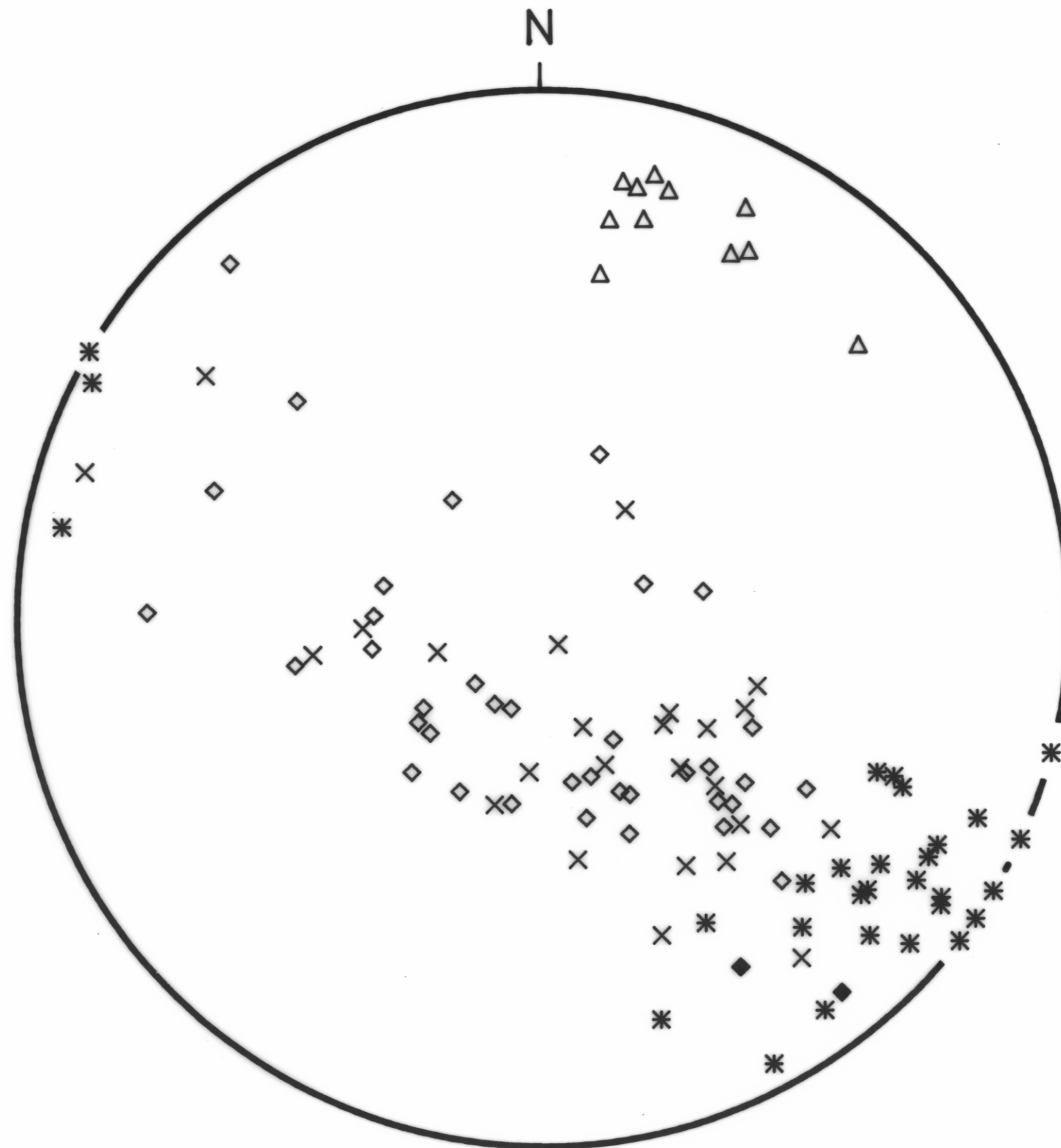
FIG. 10 Stereoplot of structural elements from domain 8
