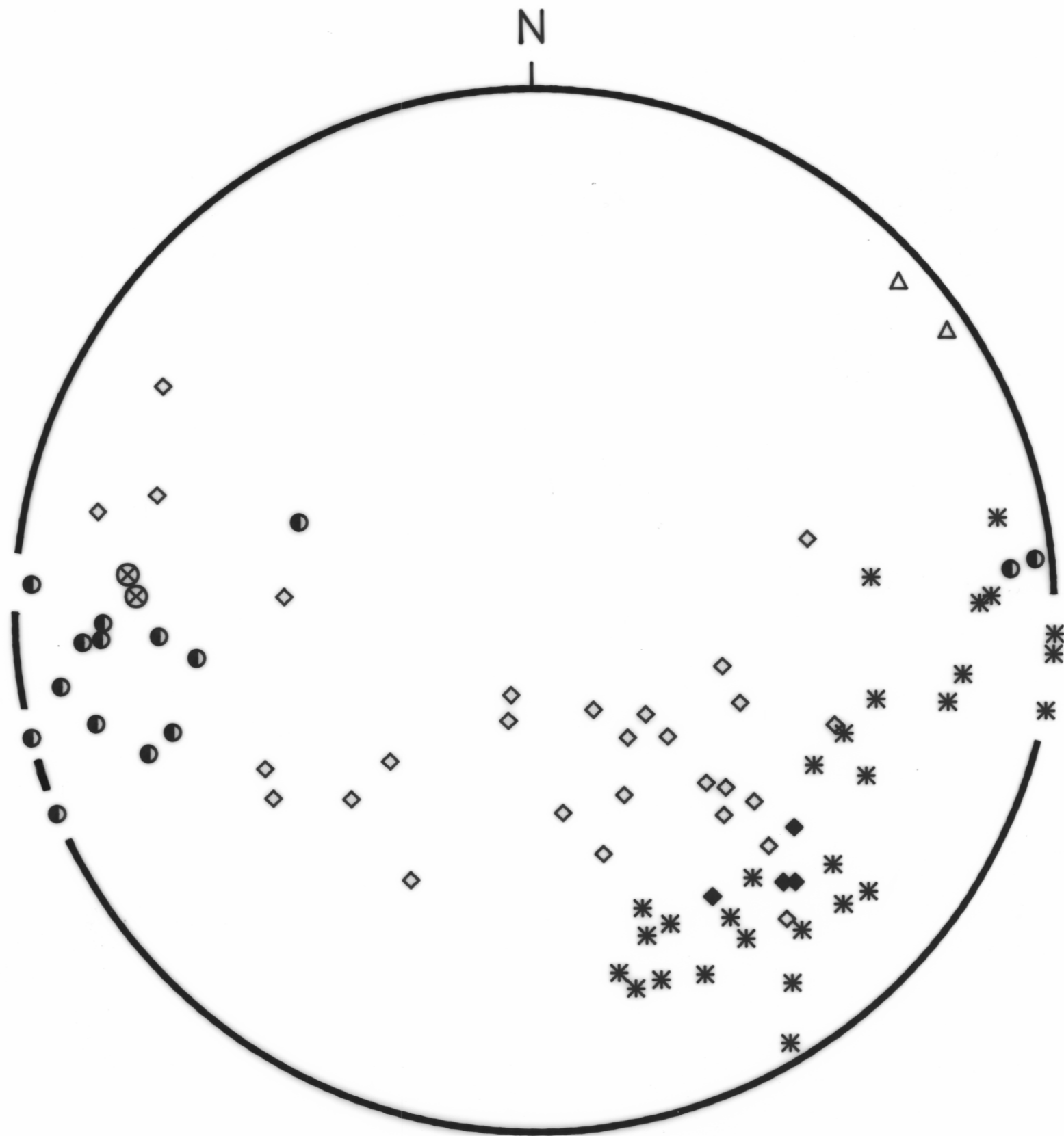
FIG. 14 Stereoplot of structural elements from domain 12
