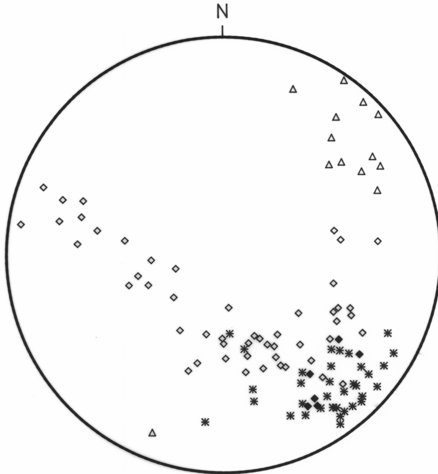
FIG. 15 Stereoplot of structural elements from domain 13
