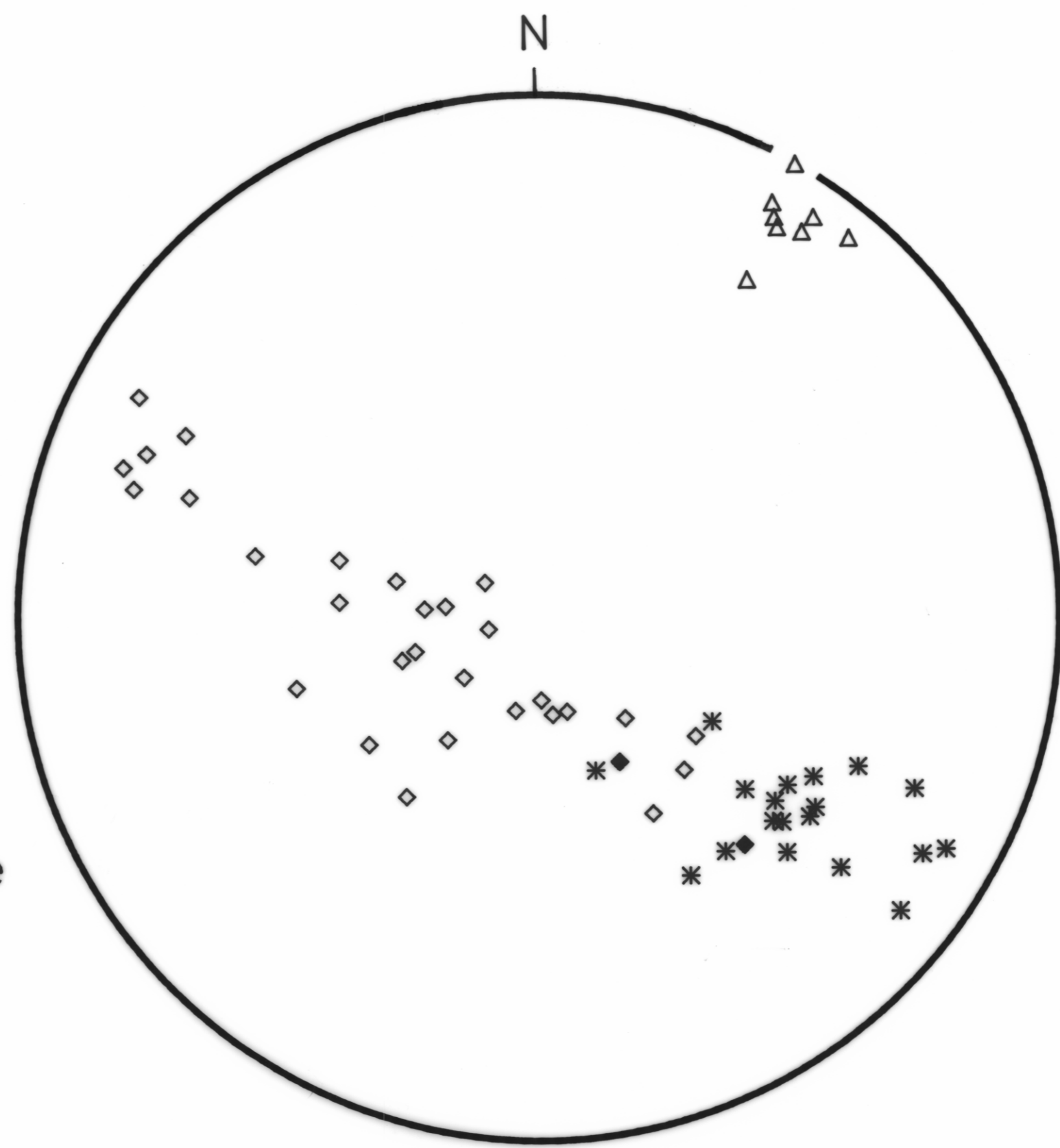
FIG. 16 Stereoplot of structural elements from domain 14
