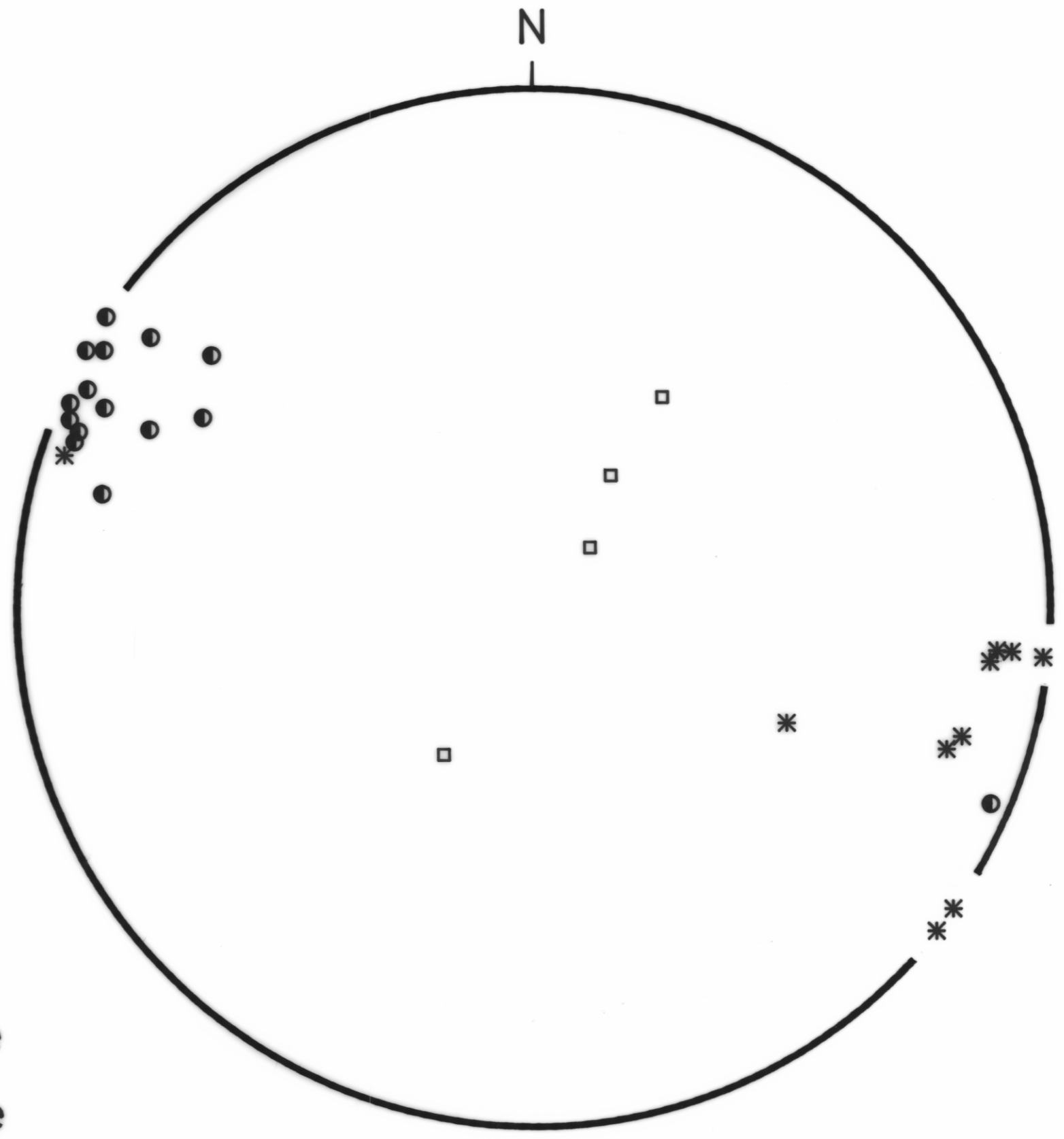
FIG. 17 Stereoplot of structural elements from domain 15
