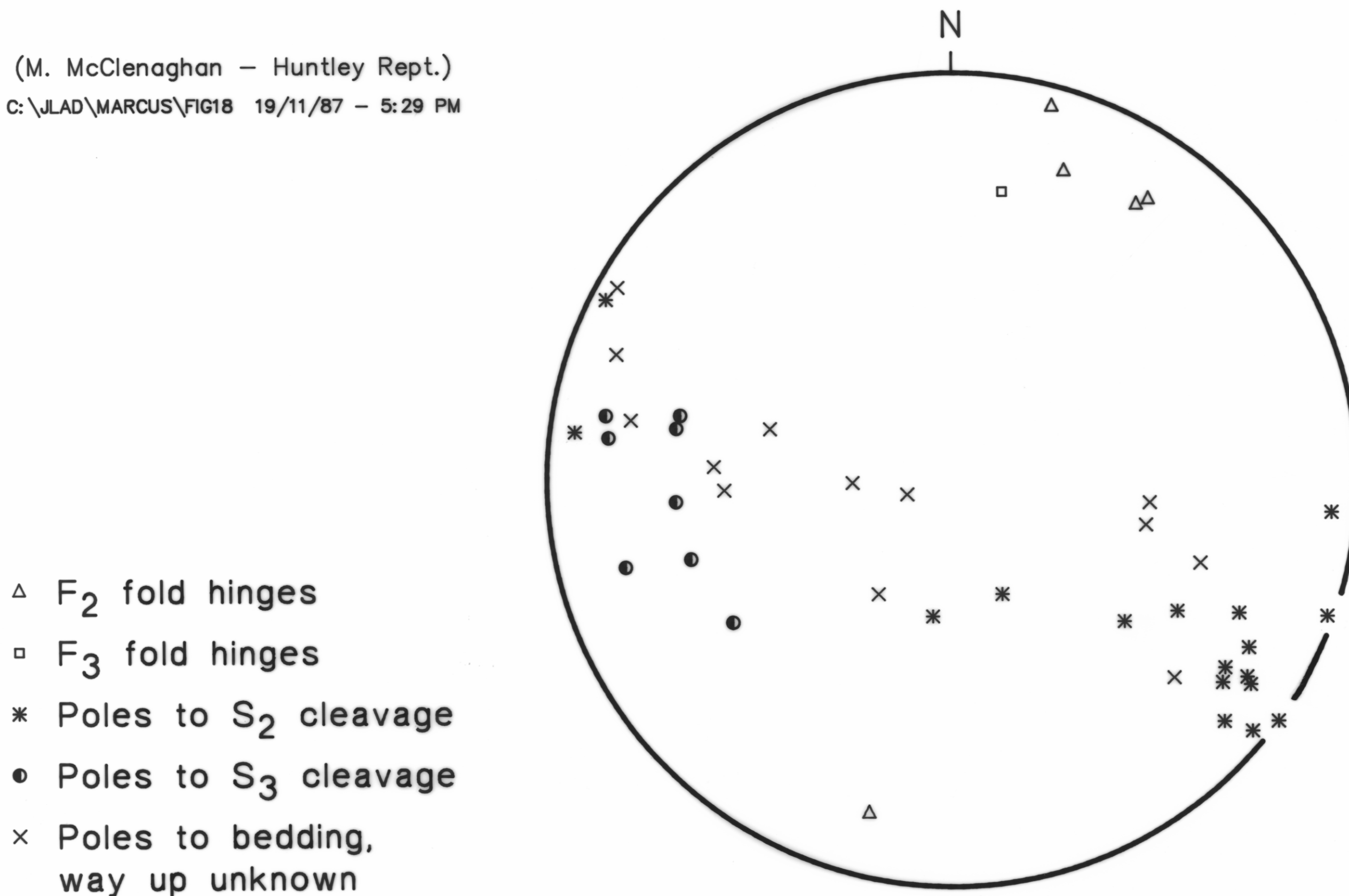
FIG. 18 Stereoplot of structural elements from domain 16
