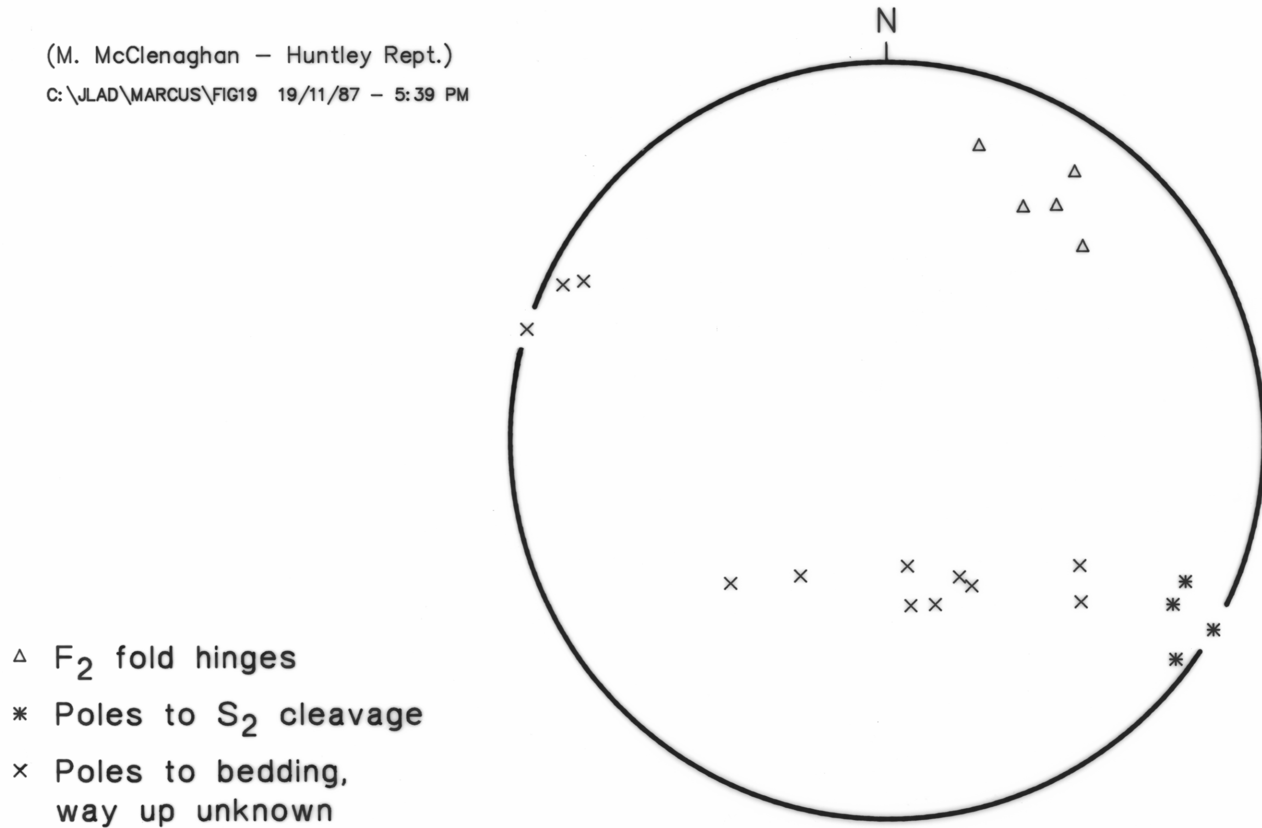
FIG. 19 Stereoplot of structural elements from domain 17
