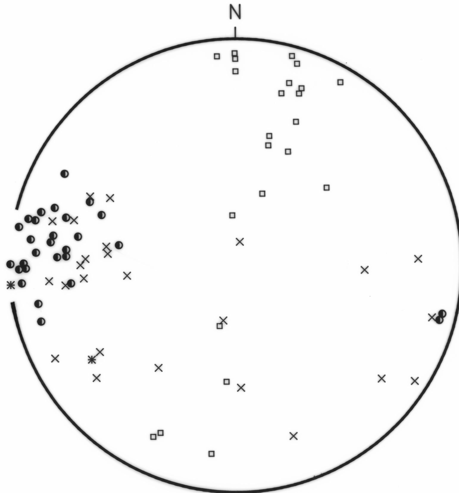
FIG. 20 Stereoplot of structural elements from domain 18
