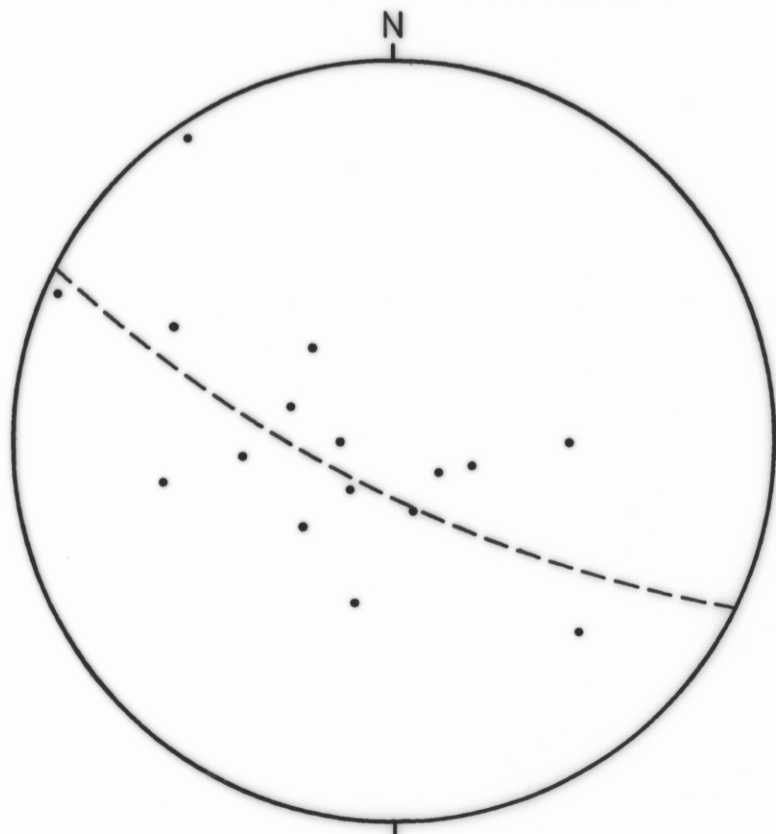
PEEGRA RD SYNFORM (CQ595570)
