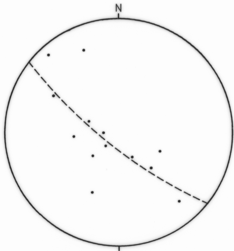
UPPER MELIN RIVULET ANTIFORM (CQ570580)
