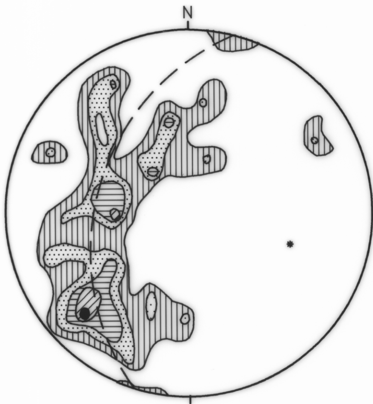
PINE CORNER RD QUARRY CONTOURED STEREOPLOT OF POLES TO BEDDING
