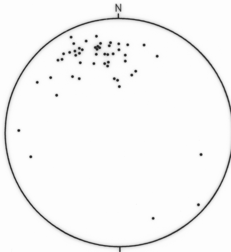
STEREOPLOTS OF POLES TO CLEAVAGE FOR 52 READINGS
