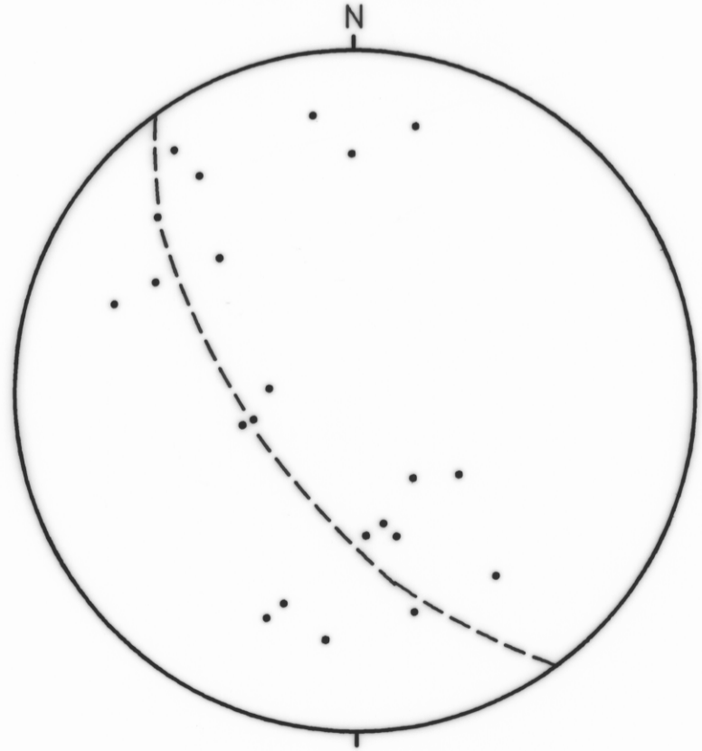
MAWBANNA SIDLING ANTIFORM
