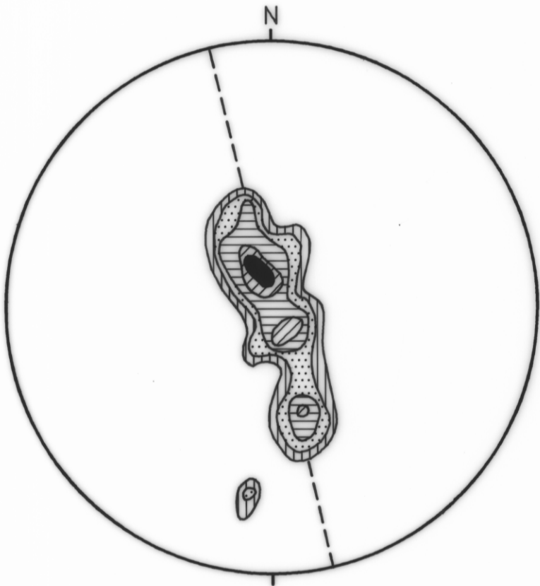
BLACK RIVER – BASS H'WAY SYNCLINE
