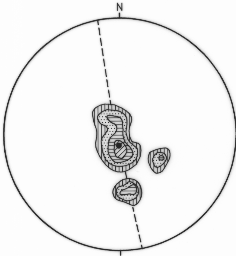
JACOBS BOAT HAROUR FAULT – BLACK RIVER ANTIFORM
