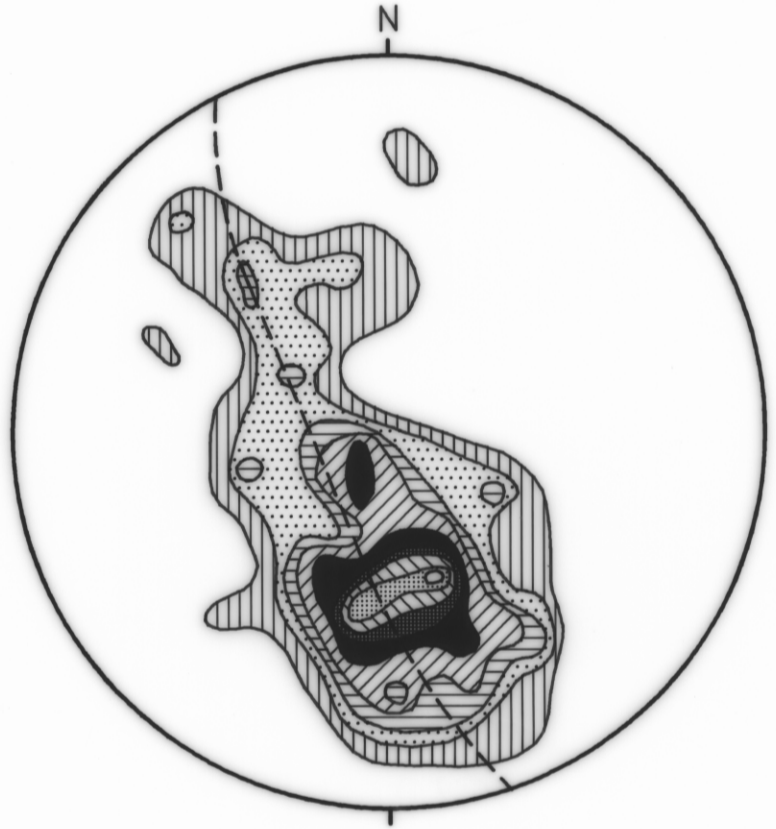
CRAYFISH CREEK ANTICLINE
