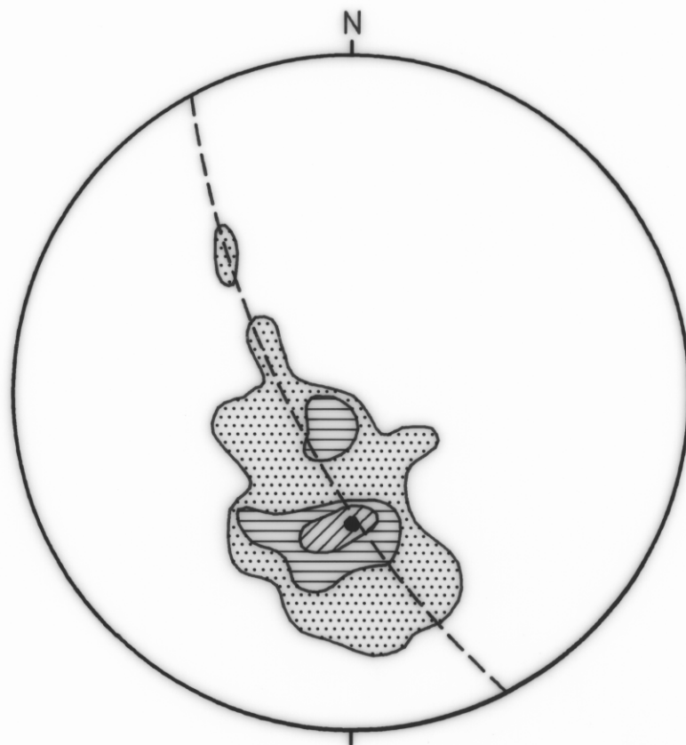
STEREOPLOT B
