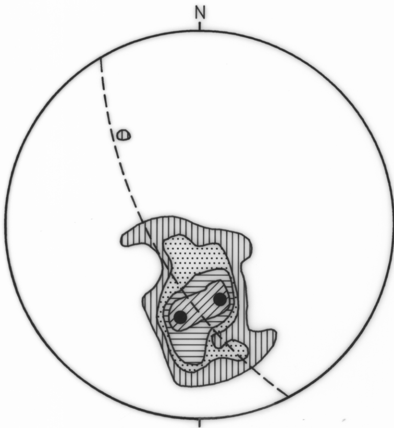
STEREOPLOT A
