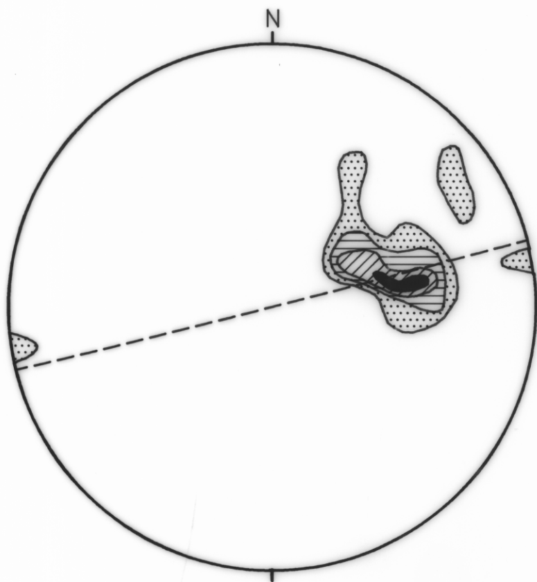
CONTOURED STEREO PLOT OF MESOSCALE FOLD HINGELINES FROM THE FORESHORE OUTCROP (CQ610763)
