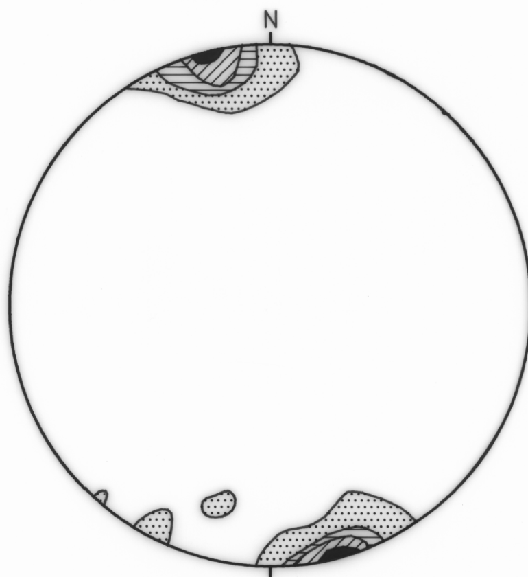
CONTOURED STEREO PLOT OF POLES TO CLEAVAGE FOR THE SAME OUTCROP (CQ734756)
