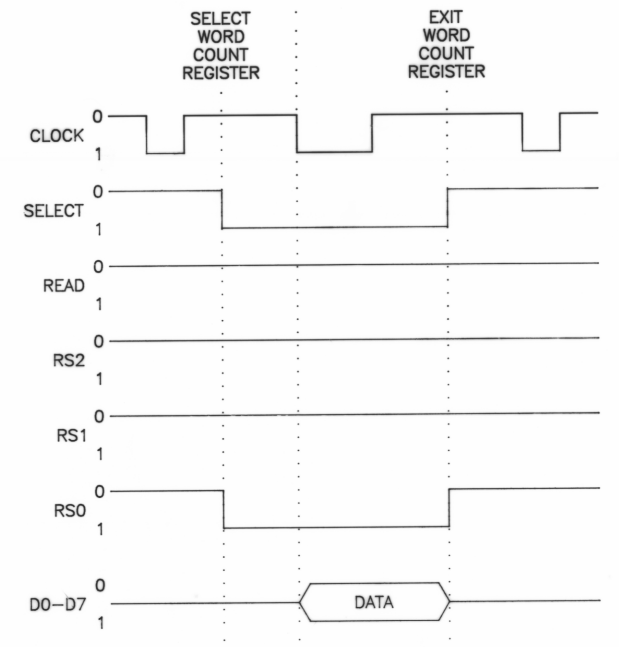
TIMING DIAGRAM FOR SELECT WORD COUNT REGISTER (6)
