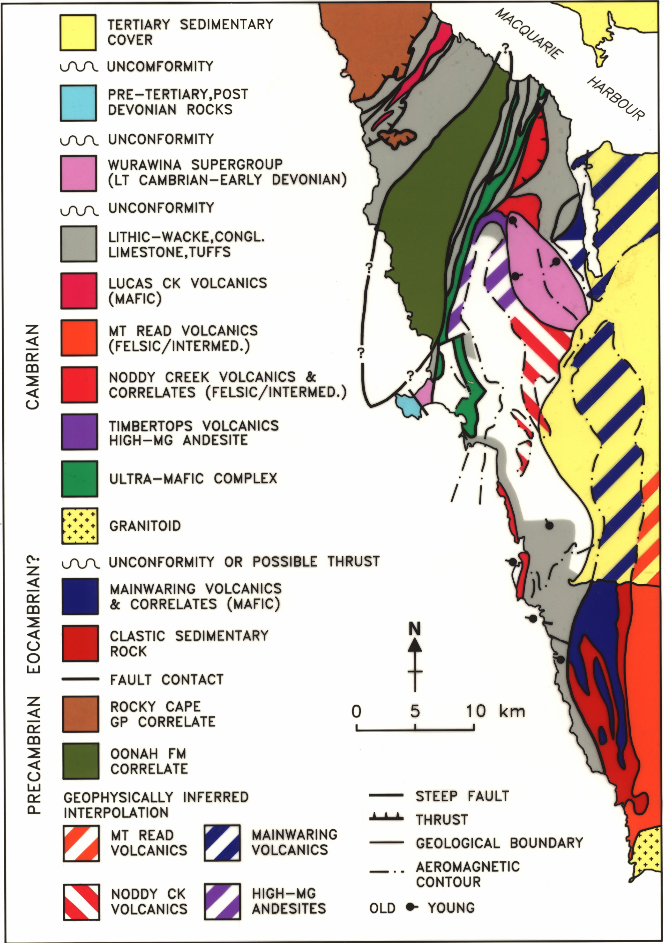
Sketch Geological Map of Sorell Peninsular to Elliot Bay Region FIGURE No. Third Italian Antarctica Symposium, Siena AUTHOR: R. Findlay TASMANIA DEPARTMENT OF MINES, DRAFTSPERSON: ASM 5307
