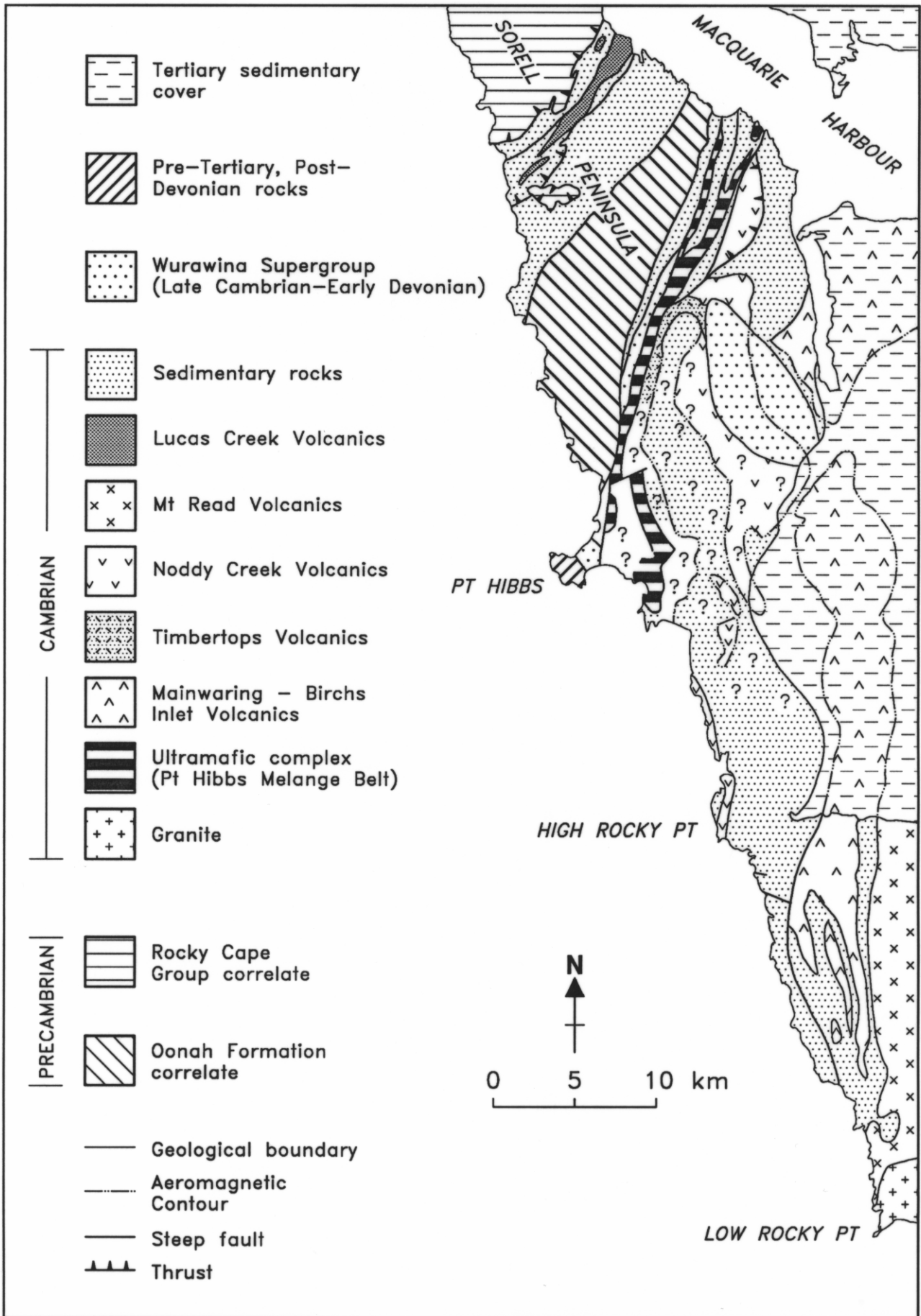
Sketch Geological Map of Sorell Peninsular to Elliot Bay Region FIGURE No. REPORT 1991/02 AUTHOR: A.V. BROWN TASMANIA DEPARTMENT OF MINES, DRAFTSPERSON: ASM 20/02/91 5307B
