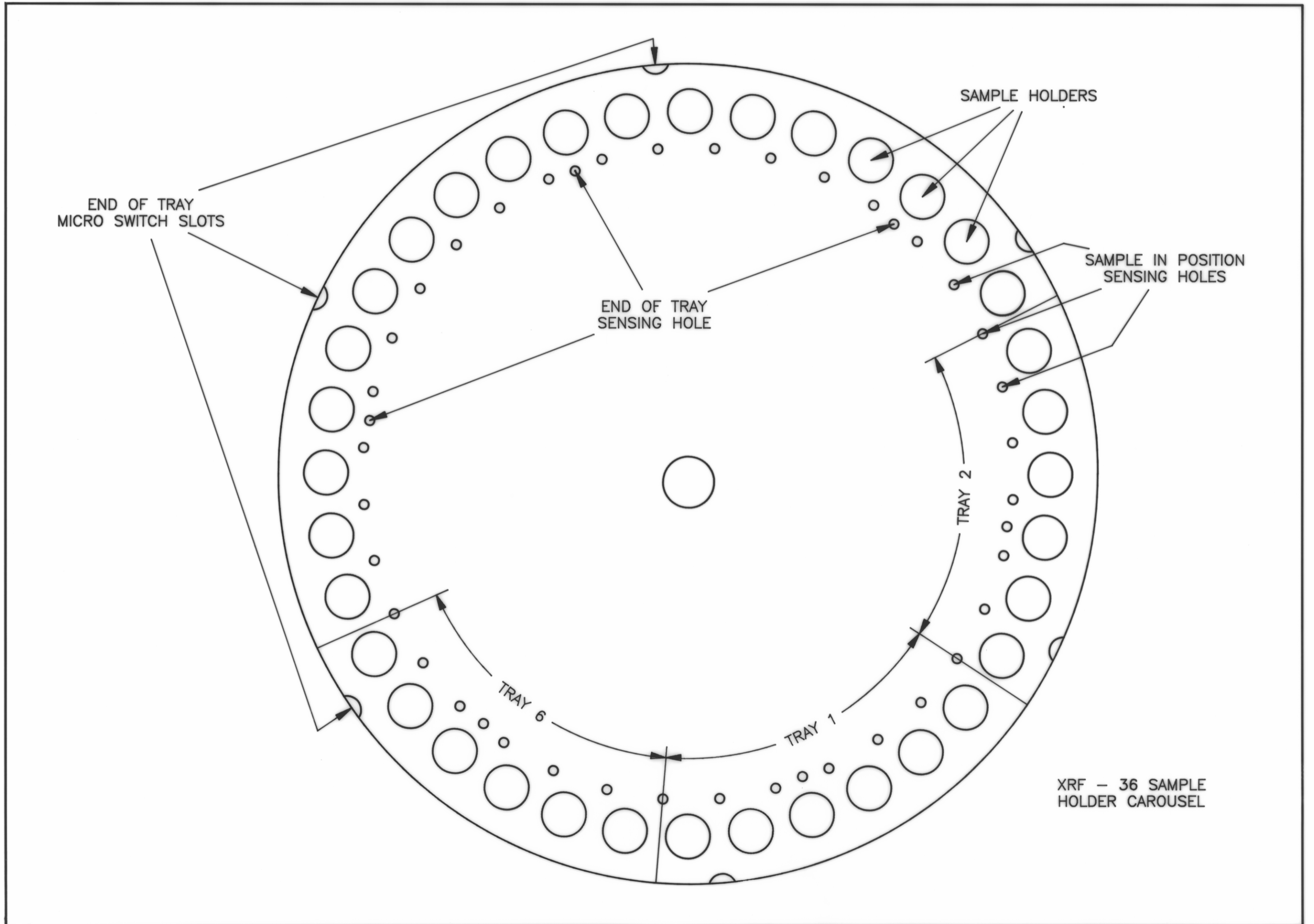
CAROUSEL U/R 1989/35 TASMANIA DEPARTMENT OF MINES, DRAFTSPERSON: ASM 09/10/89 AUTHOR: R. SEDGMAN 5310C
