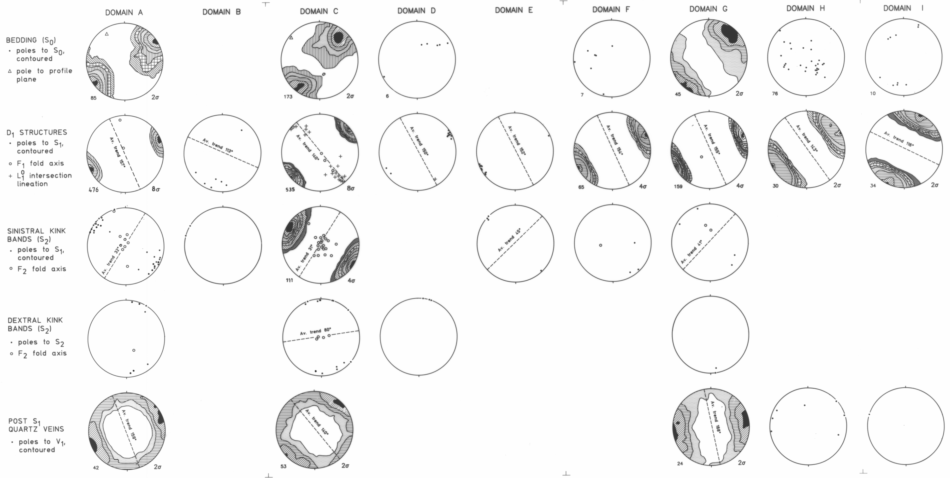
ALBERTON QUADRANGLE - STRUCTURAL DATA STEREOPLOTS FOR ALL DOMAINS FIGURE XXII U/R 1989/42 AUTHOR: B. GOSCOMBE TASMANIA DEPARTMENT OF MINES, DRAFTSPERSON: J. LADANWISKY 5313
