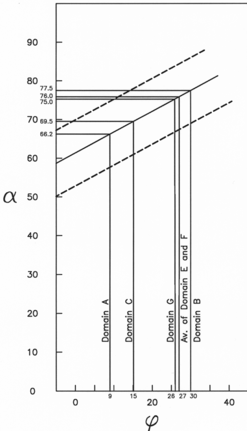
S.E. Alberton Quadrangle, Relating \alpha with \varphi after the Experimental Data of Gay & Weiss FIGURE 18 U/R 1989/42 AUTHOR: B. GOSCOMBE TASMANIA DEPARTMENT OF MINES, DRAFTSPERSON: ASM 12/10/89 5314D
