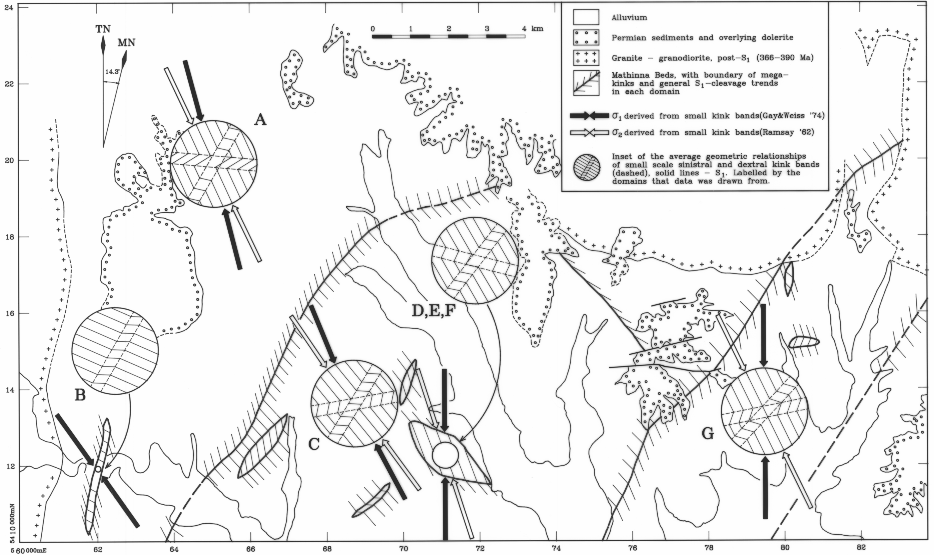
SE OF ALBERTON QUADRANGLE SUMMARY MAP OF THE AVERAGE RELATIONSHIPS BETWEEN SINISTRAL & DEXTRAL OUTCROP-SCALE KINK BANDS & \sigma_1 STRESS TENSOR IN EACH DOMAIN FIGURE 19 UNPUBLISHED REPORT 1989/42 AUTHOR: B. GOSCOMBE TASMANIA DEPARTMENT OF MINES, DRAFTSPERSON: J. LADANIWSKYJ 5314 H
