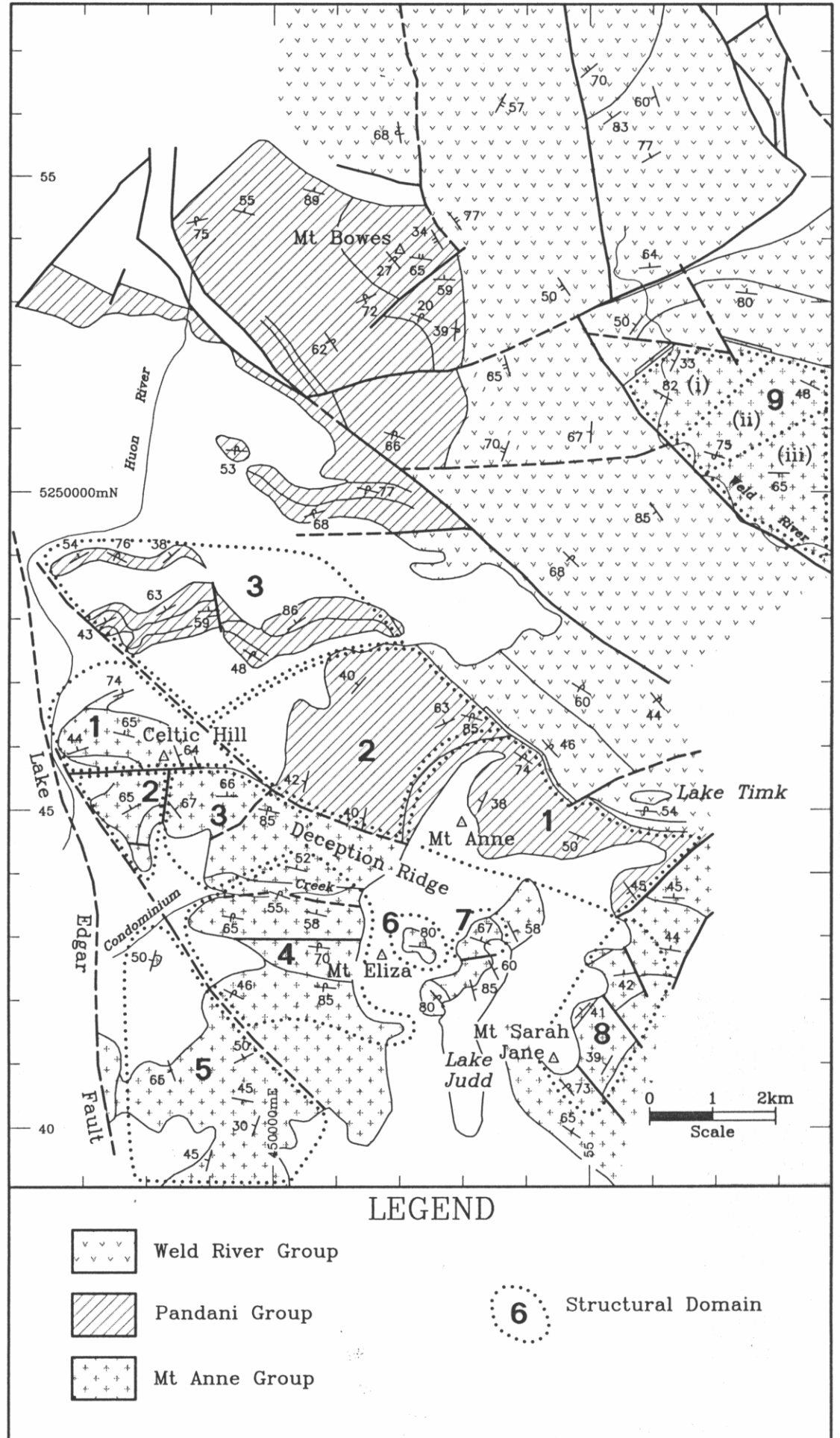
Figure C3. Structural domains, Jubilee region.
